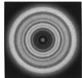
Figure 7-8 A collimated telescope should appear as a symmetrical ring pattern similar to the diffraction disk seen here.
